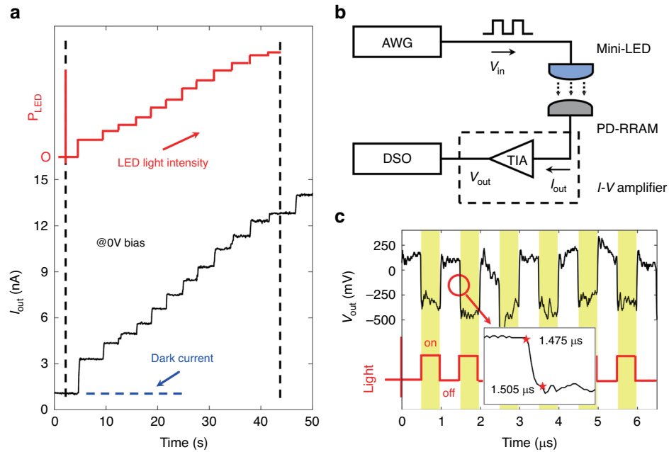
Fig. 3 Transient optoelectronic response of the PD-RRAM cell. a Measured short-circuit output current time sequence diagram. A white LED is used as the light source, with light intensity (red) ramped up from 0 to 5 \text{ mW cm}^{-2} . b Schematic illustration of the setup for speed tests. An arbitrary waveform generator (AWG) outputs a 1 MHz square wave signal to a blue Mini-LED, and the I_{out} of the PD-RRAM cell is connected to a trans-impedance amplifier (TIA) and converted into a voltage signal to be measured by the oscilloscope. c Output response of the PD-RRAM cell with the pulsed light (red line) under the short-circuit condition. The inset shows the rise and fall times of a pulse, measured between 10% and 90% of the full pulse amplitude, which are both 30 ns
