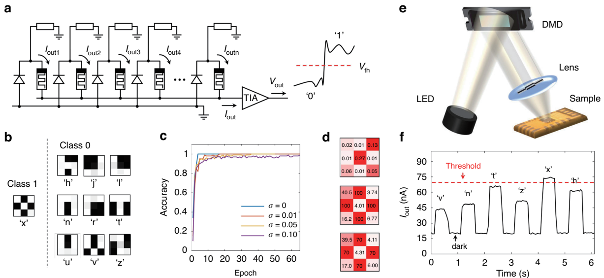
Fig. 4 A 3 \times 3 PD-RRAM array for in-sensor computing as a classifier. a Schematic illustration of the PD-RRAM array for analog MAC operations. The accumulated output current ( I_{out} ) is generated by N pixels that are connected in parallel. b Letter images of 3 \times 3 pixels used for training/inference with 2-class. c Accuracy of the classifier during training under different noise levels ( \sigma represents the variance of image noise). d From top to bottom: theoretical dimensionless weights, theoretical RRAM resistance states, actual RRAM resistance states after programming. The unit of resistance is k \Omega . e Schematic illustration of the optical setup for recognition. The LED light is spatially modulated by a DMD and resulting images are projected onto the PD-RRAM array. f Measured output of the PD-RRAM array for recognition. Projection of different letters with a duration of 0.5 s, leads to the distinct I_{out}
